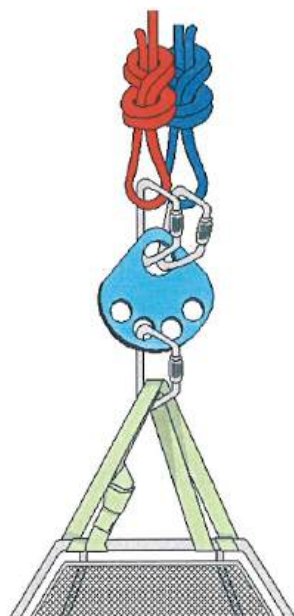
Figure 7-3: 5-foot Webbing
