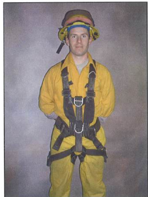
Figure 5-2: Class III Harness
