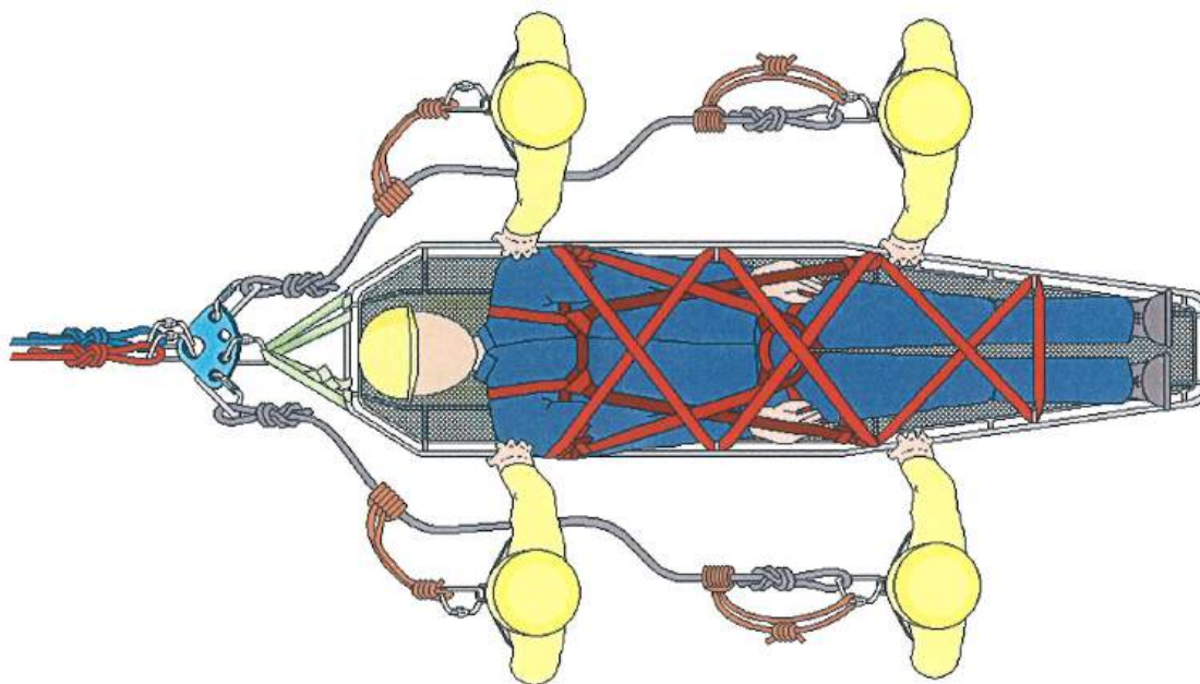
Figure 7-11: Four Rescuer Litter Attachment
