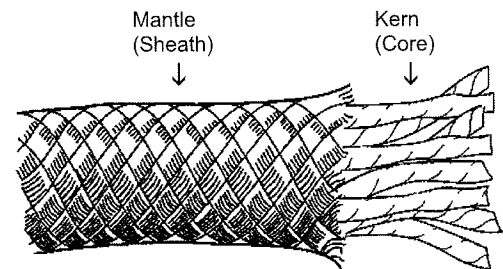
Figure 2-1: Kernmantle Rope
