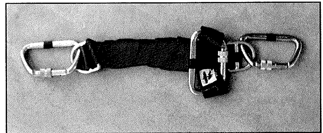
Figure 2-10: Assembled Load-releasing Device
