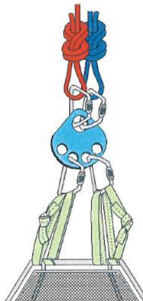
Figure 7-5: Pre-rig
