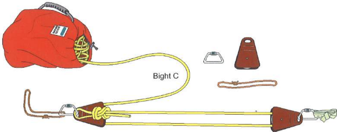
Figure 11-17: How to Construct a 5:1 Pig Rig Starting from a 3:1 Pig Rig
