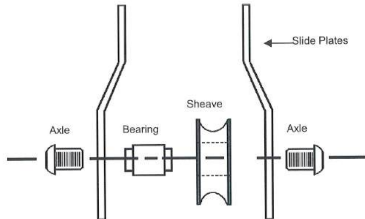
Figure 2-20: Rescue Pulley Components
