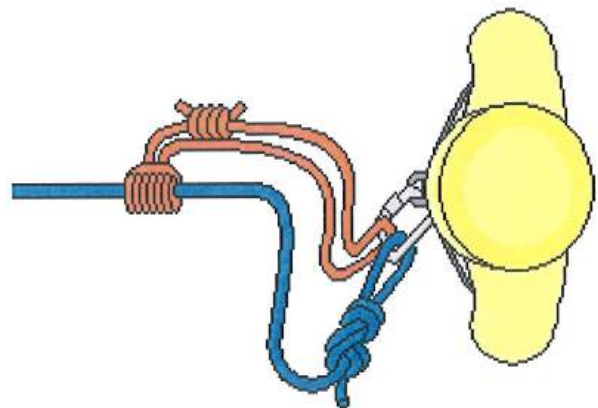
Figure 7-15: Adjustable Attachment
