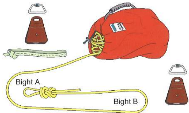
Figure 15-11: 2:1 Ladder Rig Components
