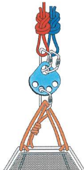
Figure 7-4: 8-foot Lifeline
