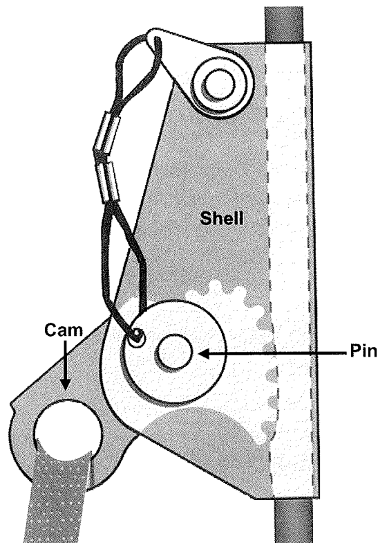
Figure 2-23: Ascender
