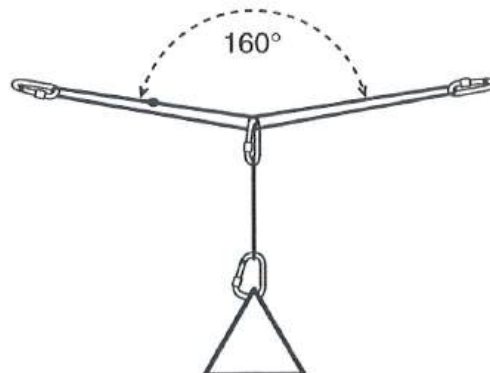
Figure 4-24: 300# Load = 1,125# at each anchor 600# Load = 2,250# at each anchor
