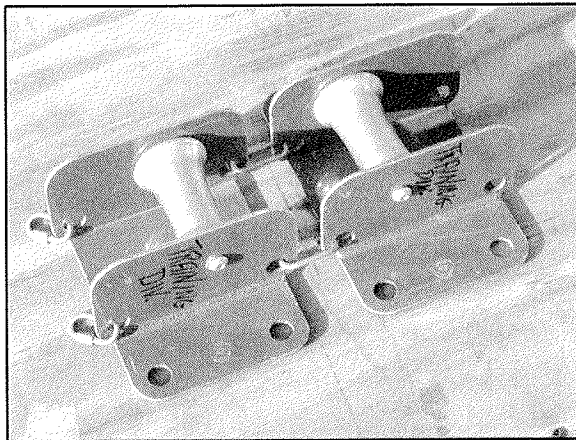
Figure 2-25: Edge Roller
