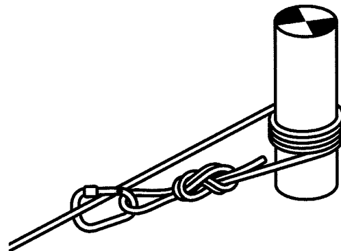
6. Tensionless Hitch
